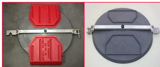
30" Vented & Non-Vented Hatch Covers
