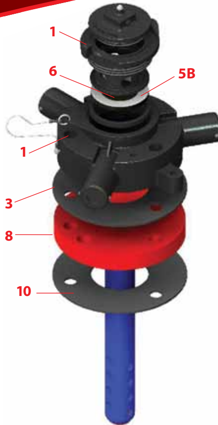
No Surge Protector in Unit. Flanged Surge Protector Below Unit.
