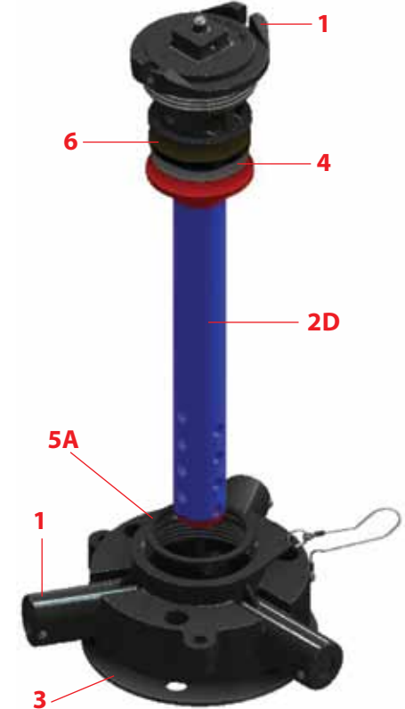
HAZARSOLVE Surge Protector, for Rubber Lined Cars
